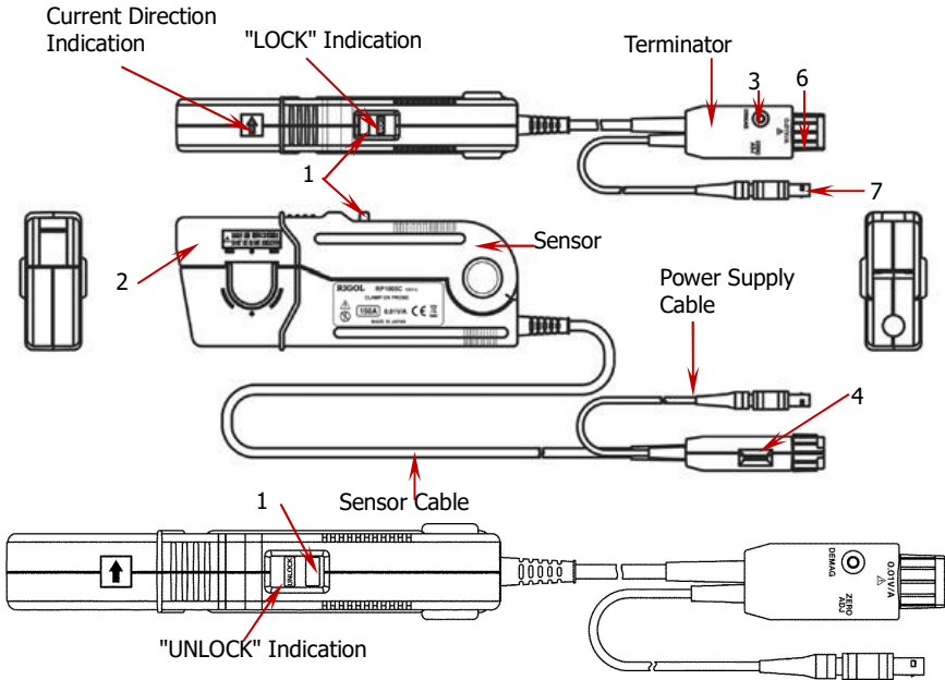
Figure 2 RP1005C/RP1006C Parts
